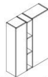
Wall cupboard: LS6V3511SA/LS6VY511SA Size: W798xD246xH1000mm
